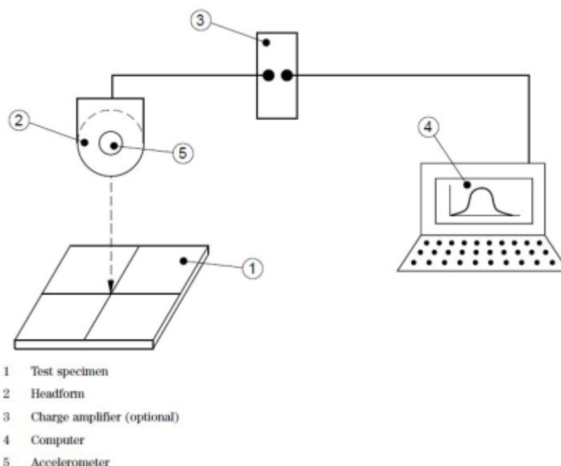
Figure 2 Apparatus for Head Impact Criteria (HIC) After SANS 51177 (2010)
