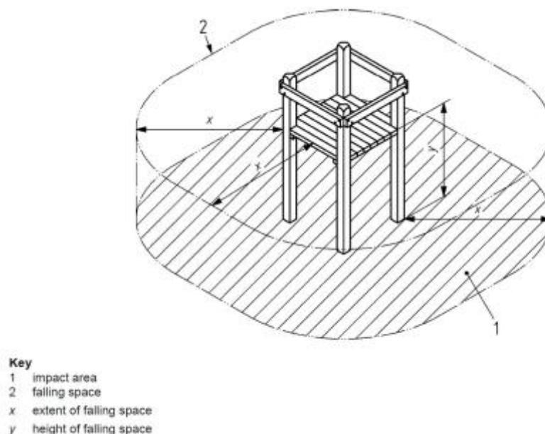
Figure 3 Falling Space Impact Area; After SANS 51176-1 (2010)
